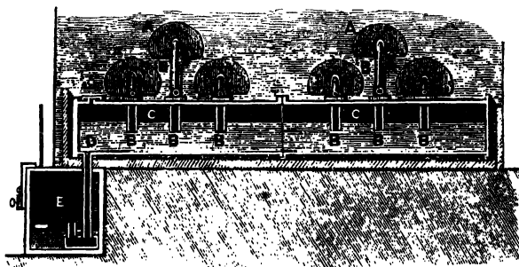
Fig. 185. A, A. The retorts. The pipes leading from the retorts marked B, C, C. The condenser of cast iron nearly filled with water into which the pipes B dip. D. Pipe through which the condensed mercury falls into the iron chest E, which is provided with a float and rod to indicate the quantity of condensed mercury.
